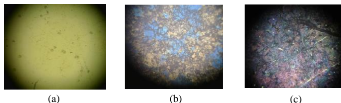
Fig. 4 Surface image of gold QCM sensor (a); polyaniline modified gold QCM sensor (b); polyaniline-nickel compound modified gold QCM sensor (c).
