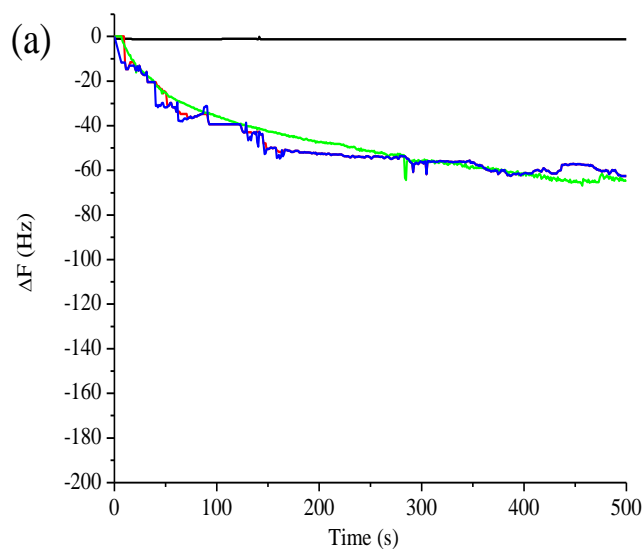
Fig. 8 Real time signal responses of polyaniline/nickel compound modified gold QCM sensor in commercial hard capsule sample solution.
