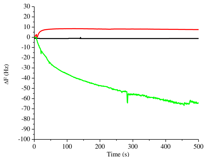
Fig. 6 Real time signal responses of polyaniline/nickel compound modified gold QCM sensor in demineralized water (black), 100 ppm bovine gelatin (green) and 100 ppm porcine gelatin (red) solution. The experiments were performed at room temperature.
