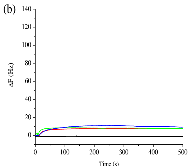
Fig. 7 Real time signal responses of polyaniline/nickel compound modified gold QCM sensor in 100 ppm bovine gelatin (a) and porcine gelatin (b). The experiments were performed at room temperature and repeated three times. Black lines in (a) and (b) are blank solution (demineralized water) responses. Red lines, blue lines, and green lines in (a) and (b) are the signal responses from the first, second, and third measurements, respectively.
