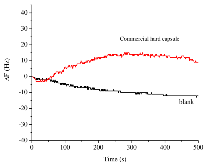
Fig. 8 Real time signal responses of polyaniline/nickel compound modified gold QCM sensor in commercial hard capsule sample solution.
