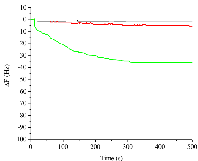
Fig. 5 Real time signal responses of unmodified gold QCM sensor in demineralized water (black), 100 ppm bovine gelatin (green) and 100 ppm porcine gelatin (red) solution. The experiments were performed at room temperature.
