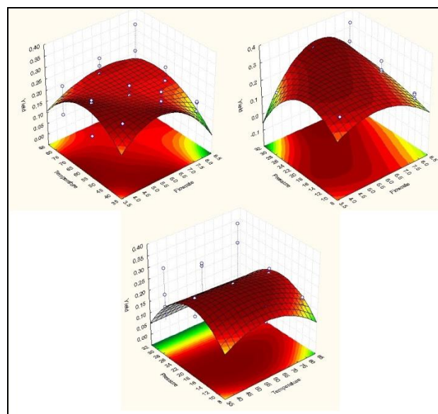
Fig. 4 Three-dimensional plot of the response surface for global oil yields of Piper Betle leaves
