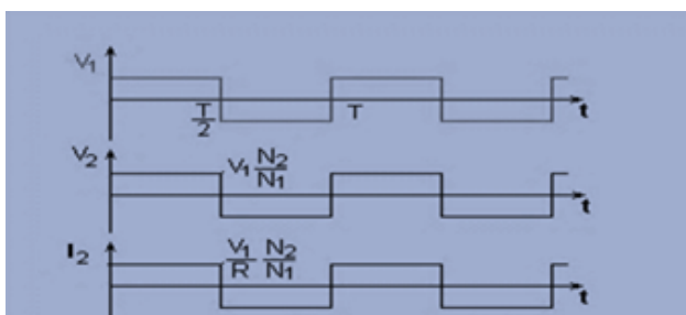
Fig. 4 High Frequency Transformer.
