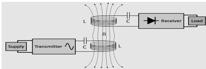
Fig. 3 Schematic diagram for Wireless power transfer [12].
