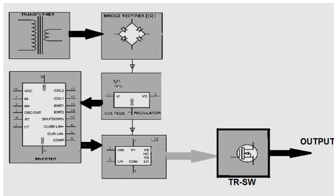
Fig. 8 Schematic diagram for 12v dc transmitter[21].
