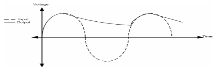
Fig. 6 Output the half-wave Rectifier.
