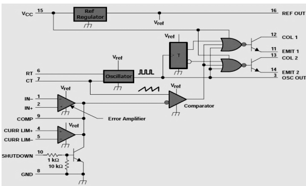
Fig. 8 Pulse width modulator typical circuit [10].
