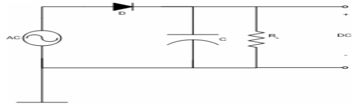
Fig. 5 Electronic circuit for half wave Rectifiers.
