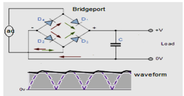
Fig. 7 Full wave Rectifiers Circuit and waveform.
