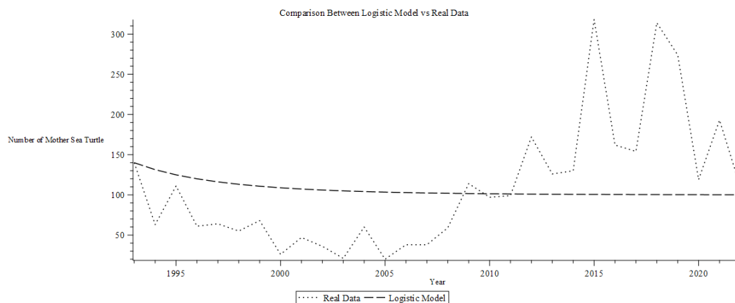
Figure 3. Logistic model fitted on actual data points
