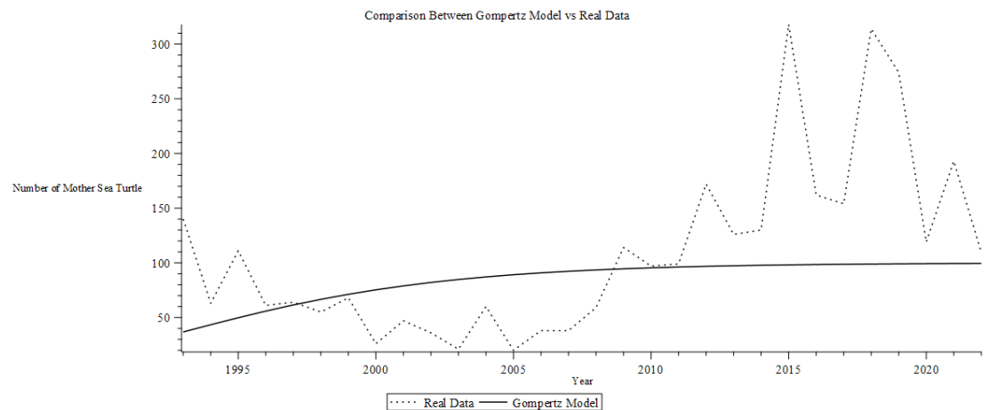
Figure 4. Gompertz model fitted on actual data points
