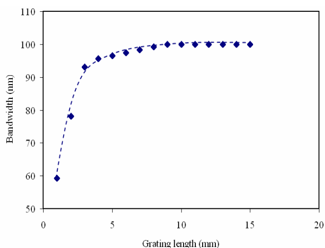
Fig. 5. The relationship between fiber grating sensor bandwidth and grating lengths.
