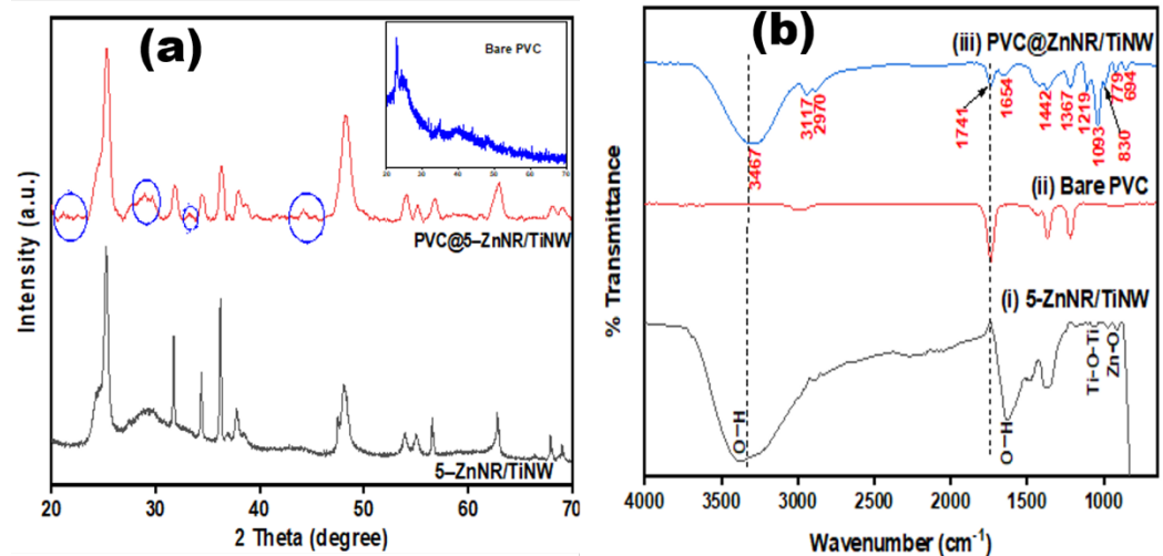
Figure 1. (a) XRD and (b) ATR-FTIR spectra of PVC supported ZnNR/TiNW compared with unsupported, and with bare PVC (inset)
