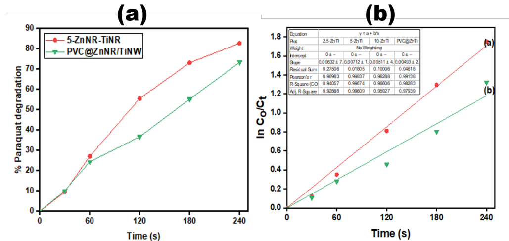
Figure 4. (a) Photocatalytic degradation (%) of paraquat dichloride under UV light irradiation, over unsupported ZnNR/TiNW and supported PVC@ZnNR/TiNW, and (b) Kinetic Linear Fit of paraquat photocatalytic degradation under UV irradiation, of unsupported compared with PVC supported ZnNR/TiNW
