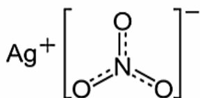
Fig. 2 Molecular structure of silver nitrate.
