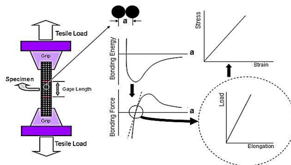
Fig 4 Schematic of tensile test.
