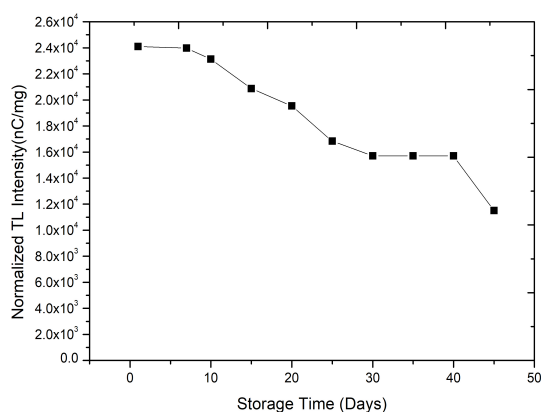
Figure 4 Fading for fabricated Ge-B doped flat fibers under normal ambient conditions.
